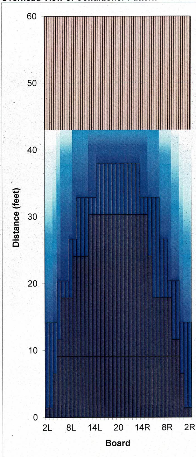
パターン1 Overhead View of Conditioner Pattern
